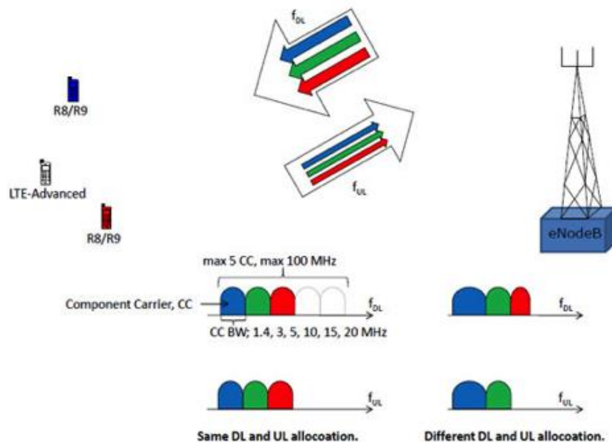
Figure 5: Carrier Aggregation (FDD)
