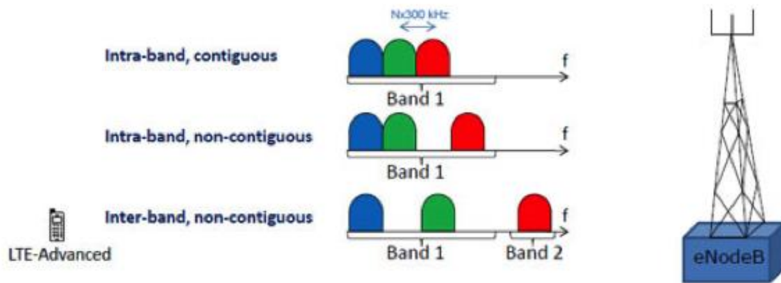
Figure 6: Carrier Aggregation intra-band and inter-band aggregation alternatives
